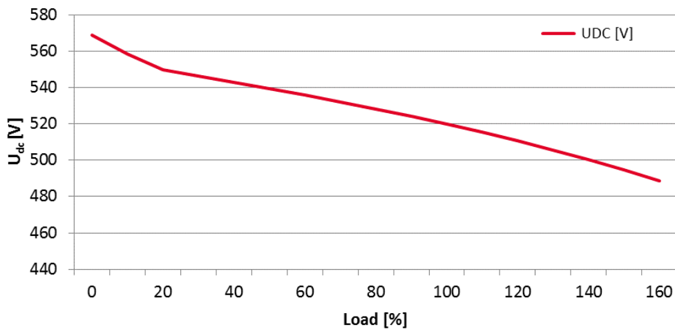
Figure 7 Drive dc-link voltage vs. load (diode rectifier front-end, with FN3440 series)
