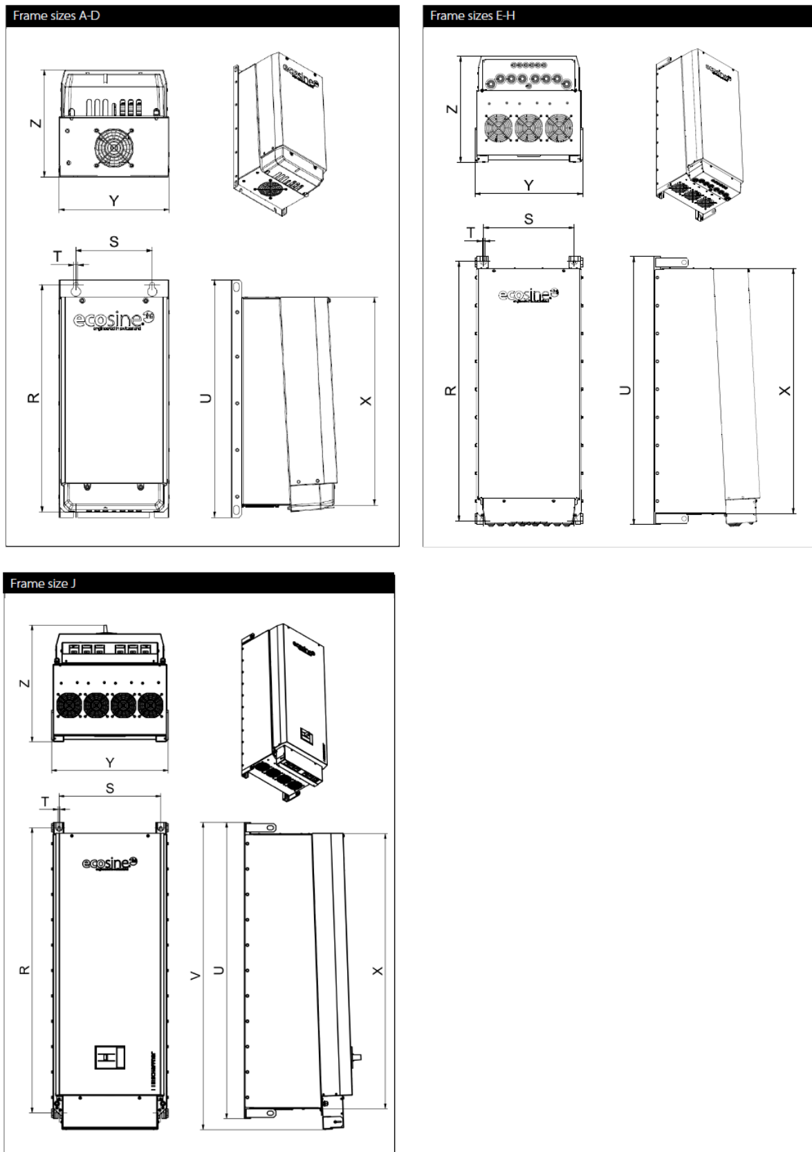
Figure 4 Mechanical Data of FN3440, FN3450, FN3442 and FN3452
