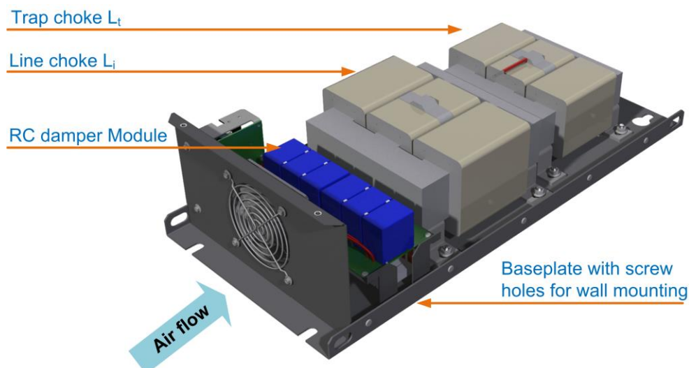
Figure 13 Lower-stage of Ecosine Evo filter (Type E0FAJRX, frame size D): lower-stage
