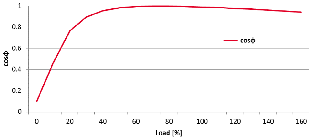
Figure 6 Power factor vs. load (diode rectifier front-end)
