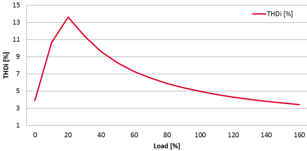
Figure 5 THDi vs. load (diode rectifier front-end)
